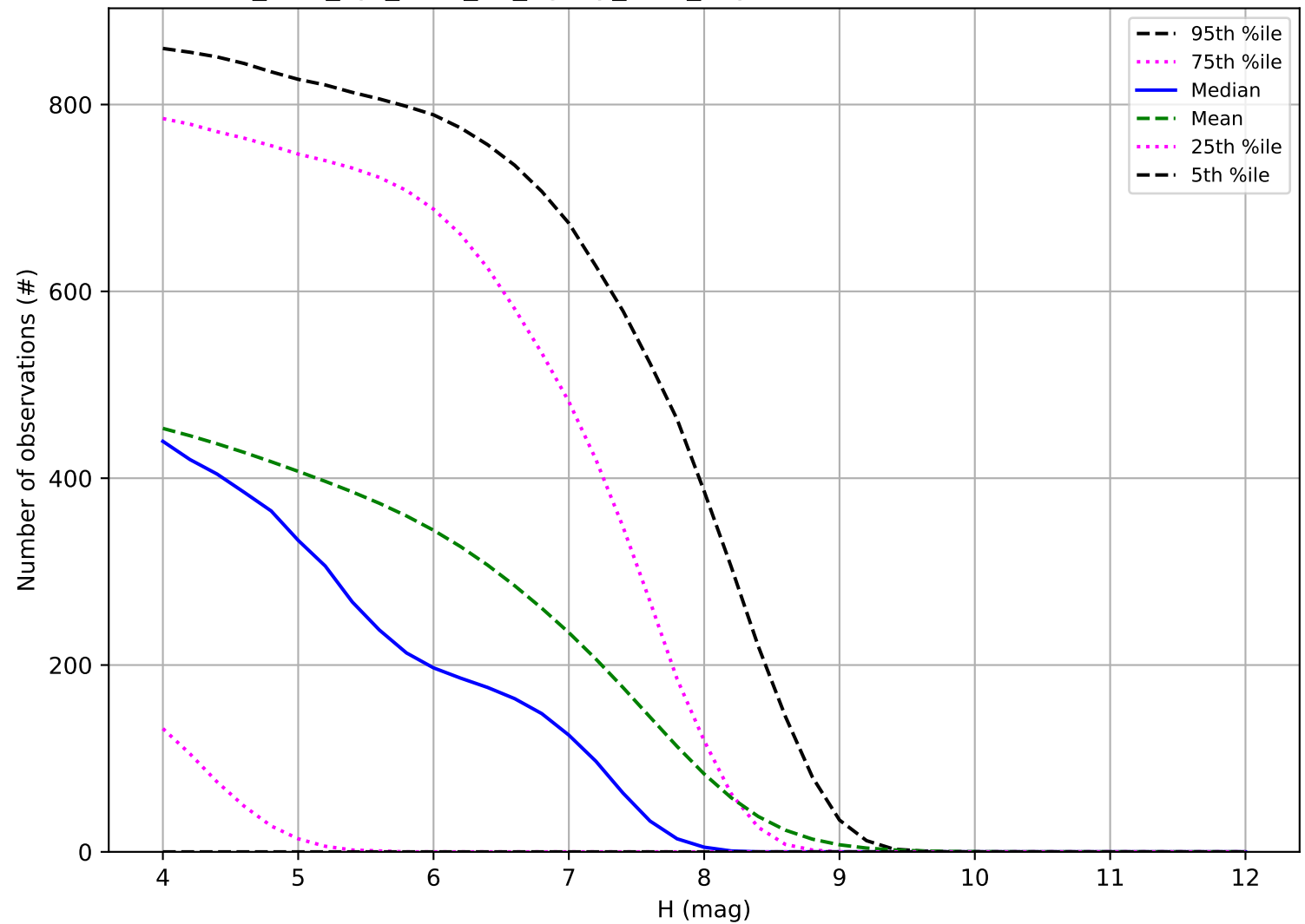
too_elab_2yr_r128_d3_ugrizy_v3.4_10yrs: Number of observations TNO
