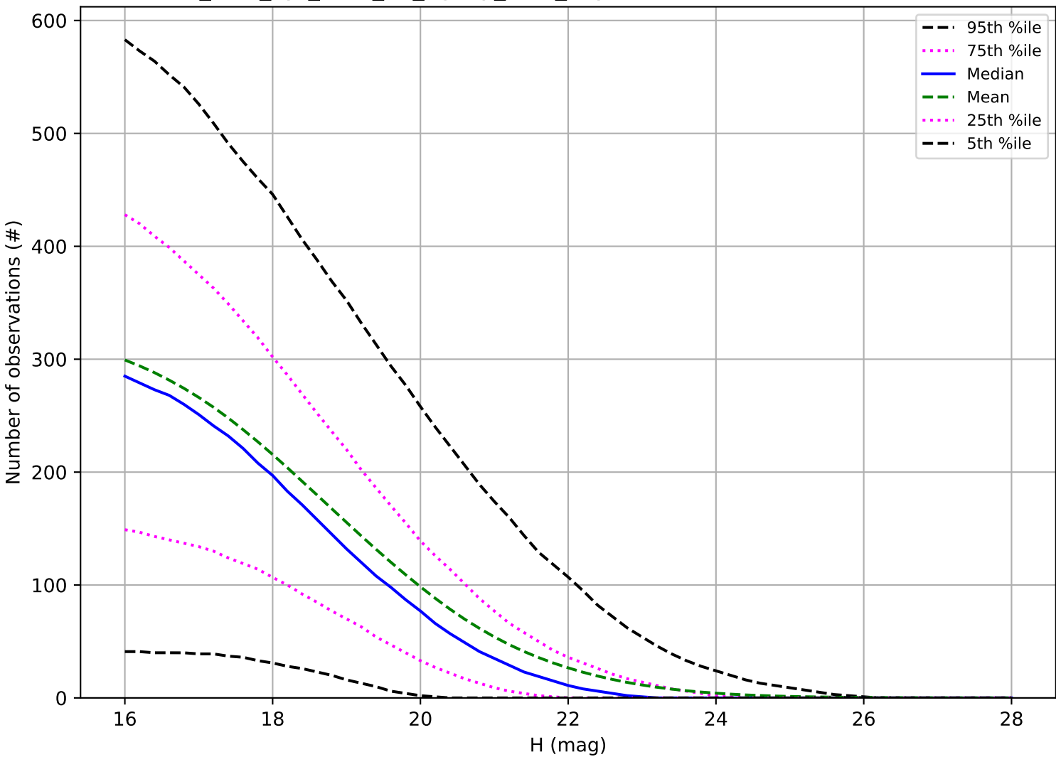
too_elab_2yr_r128_d3_ugrizy_v3.4_10yrs: Number of observations PHA
