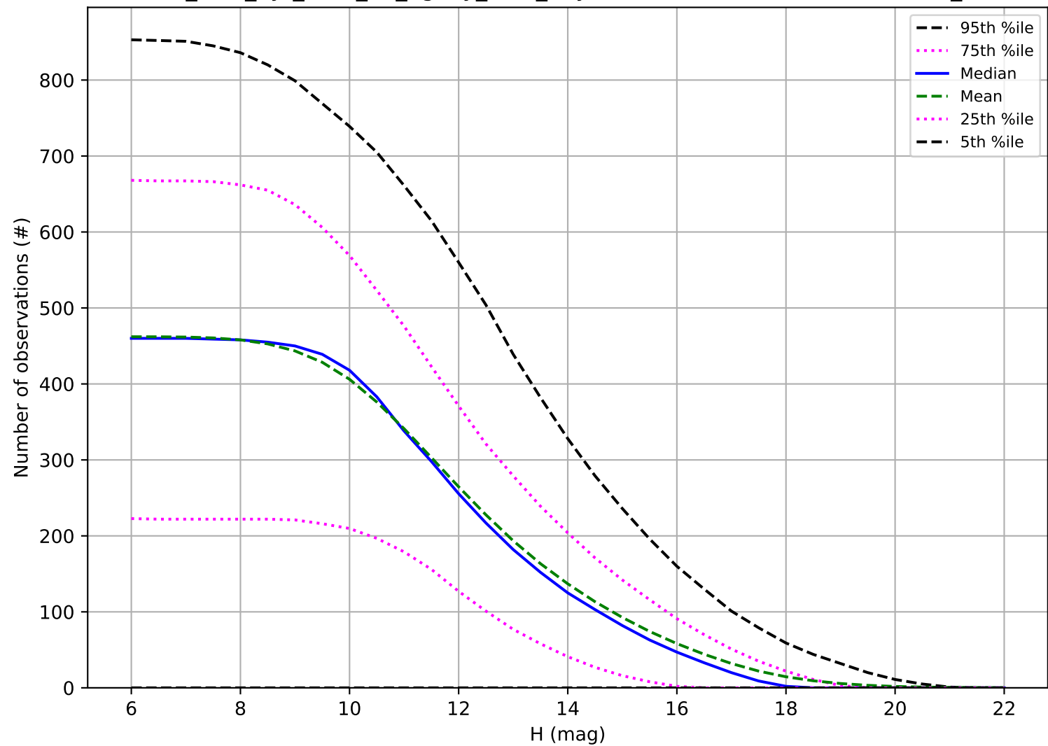
too_elab_2yr_r128_d3_ugrizy_v3.4_10yrs: Number of observations OCC_r5
