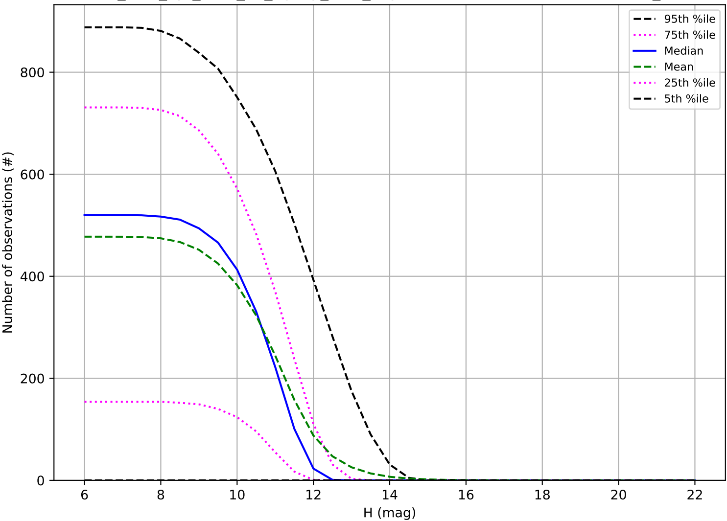
too_elab_2yr_r128_d3_ugrizy_v3.4_10yrs: Number of observations OCC_r20
