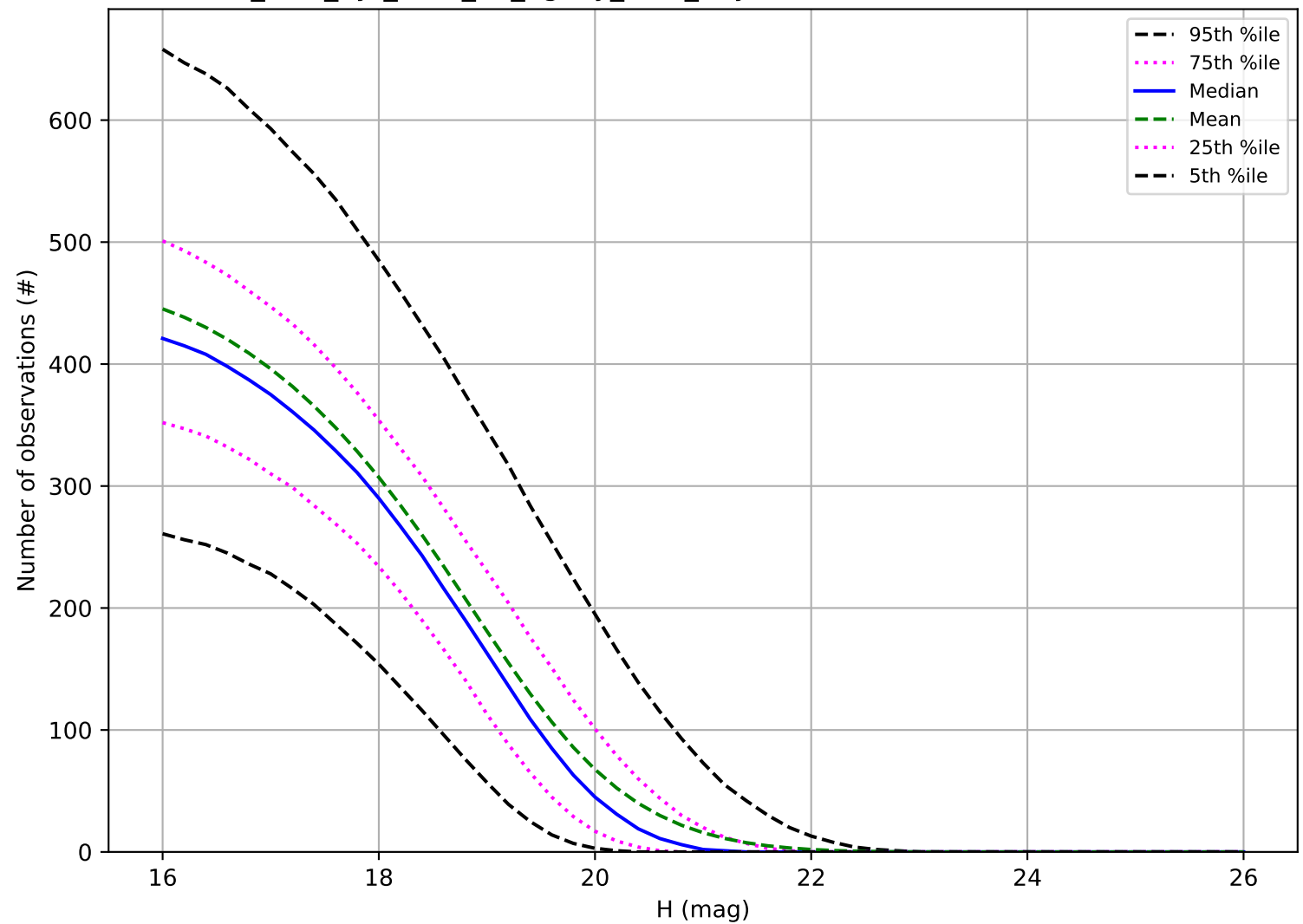
too_elab_2yr_r128_d3_ugrizy_v3.4_10yrs: Number of observations MBA
