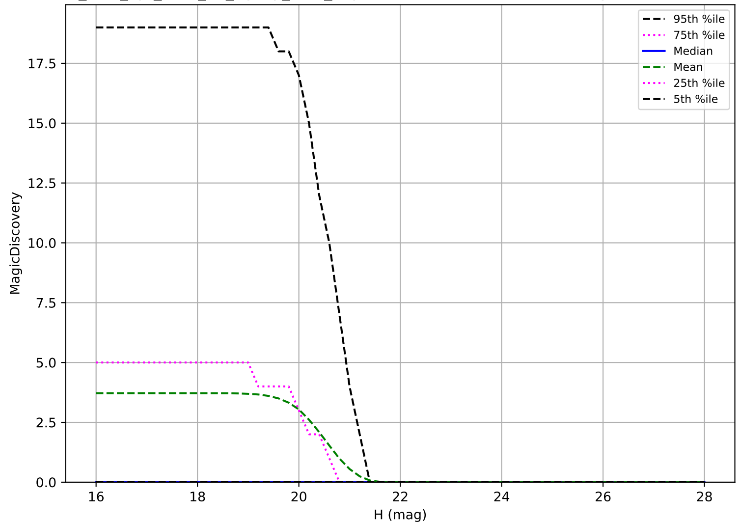
too_elab_2yr_r128_d3_ugrizy_v3.4_10yrs: Vatira 6 detections in 60 nights detection loss
