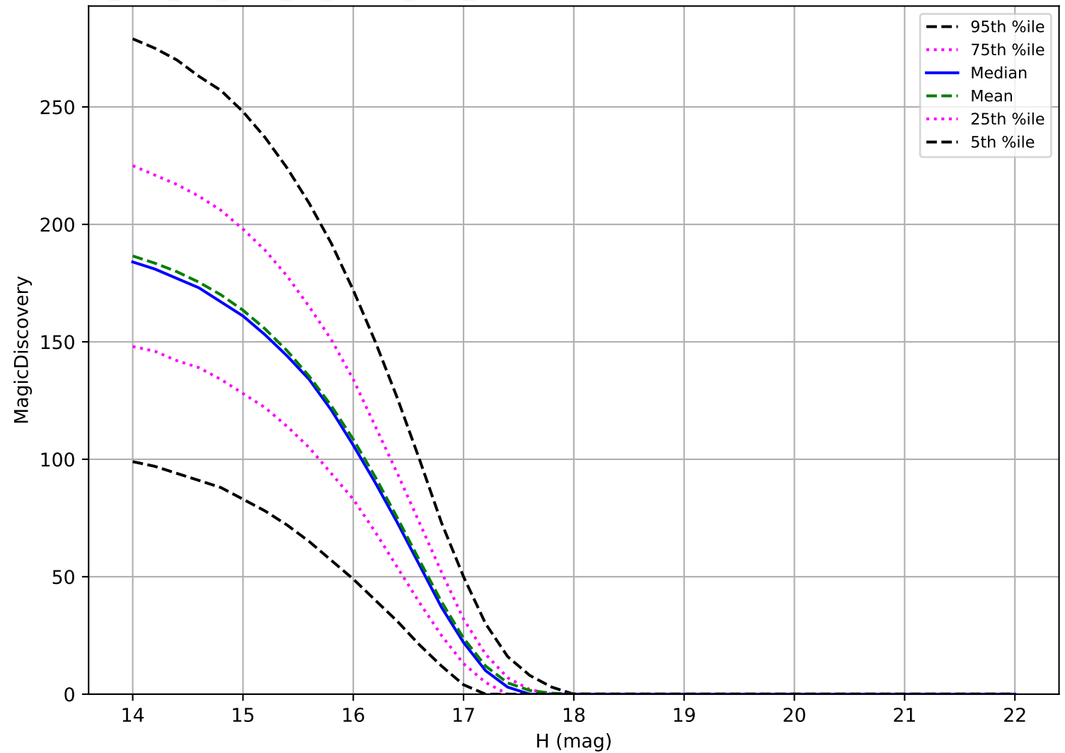
too_elab_2yr_r128_d3_ugrizy_v3.4_10yrs: Trojan 6 detections in 60 nights detection loss
