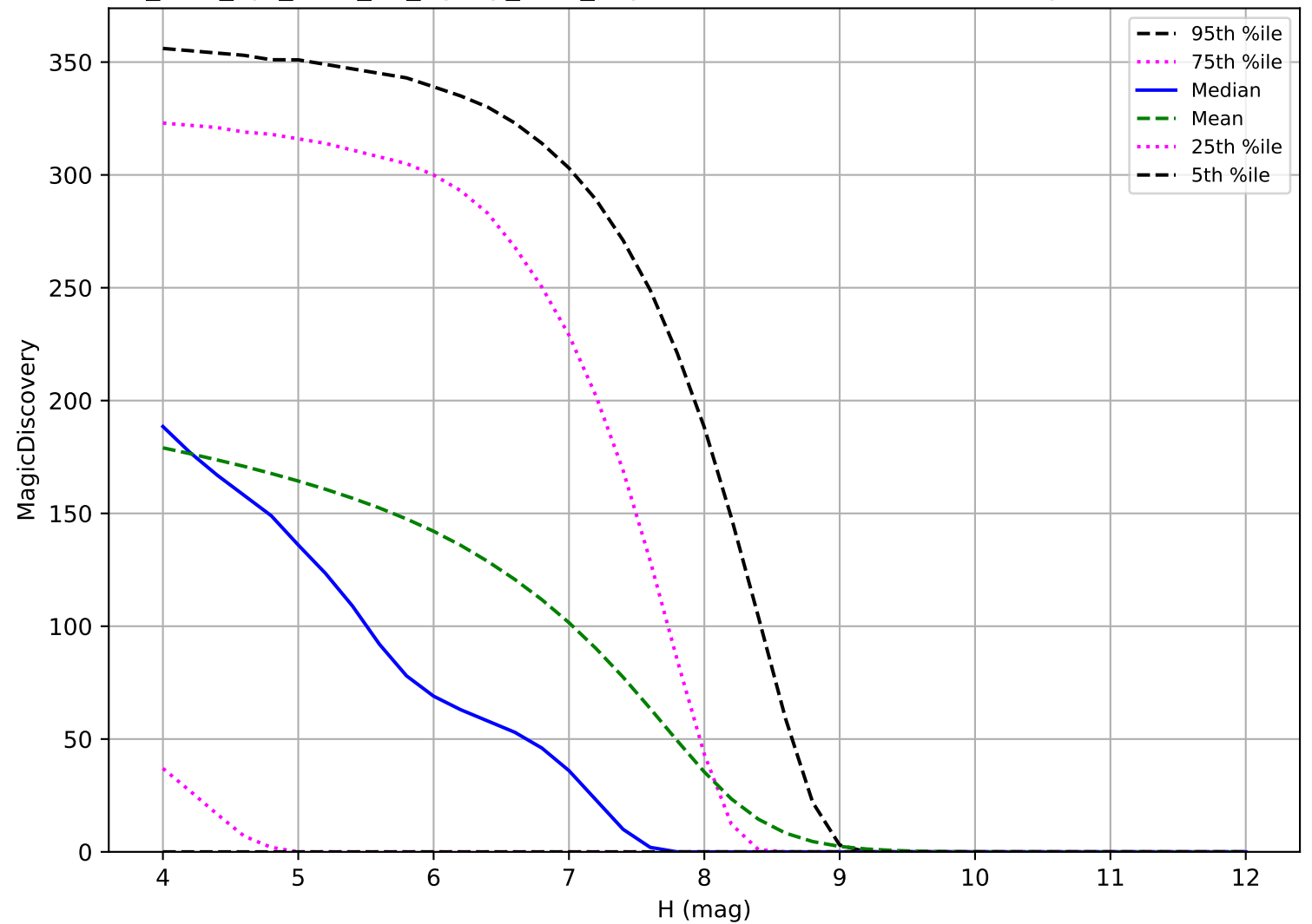
too_elab_2yr_r128_d3_ugrizy_v3.4_10yrs: TNO 6 detections in 60 nights detection loss
