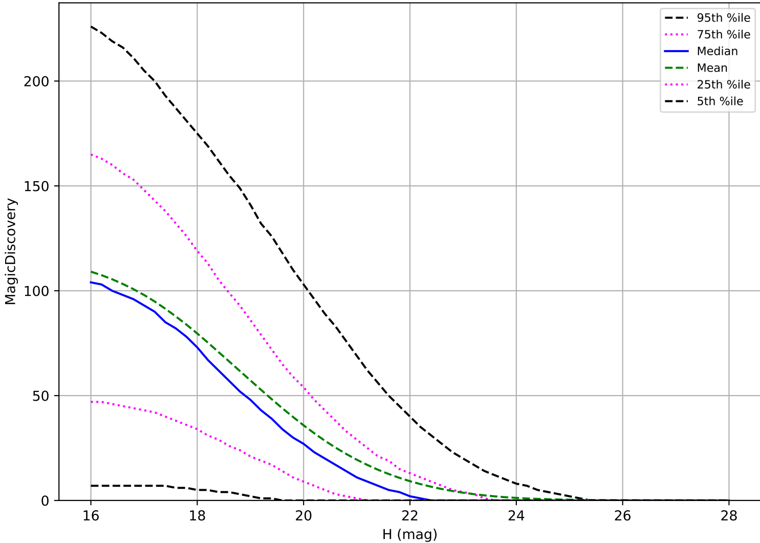
too_elab_2yr_r128_d3_ugrizy_v3.4_10yrs: PHA 6 detections in 60 nights detection loss
