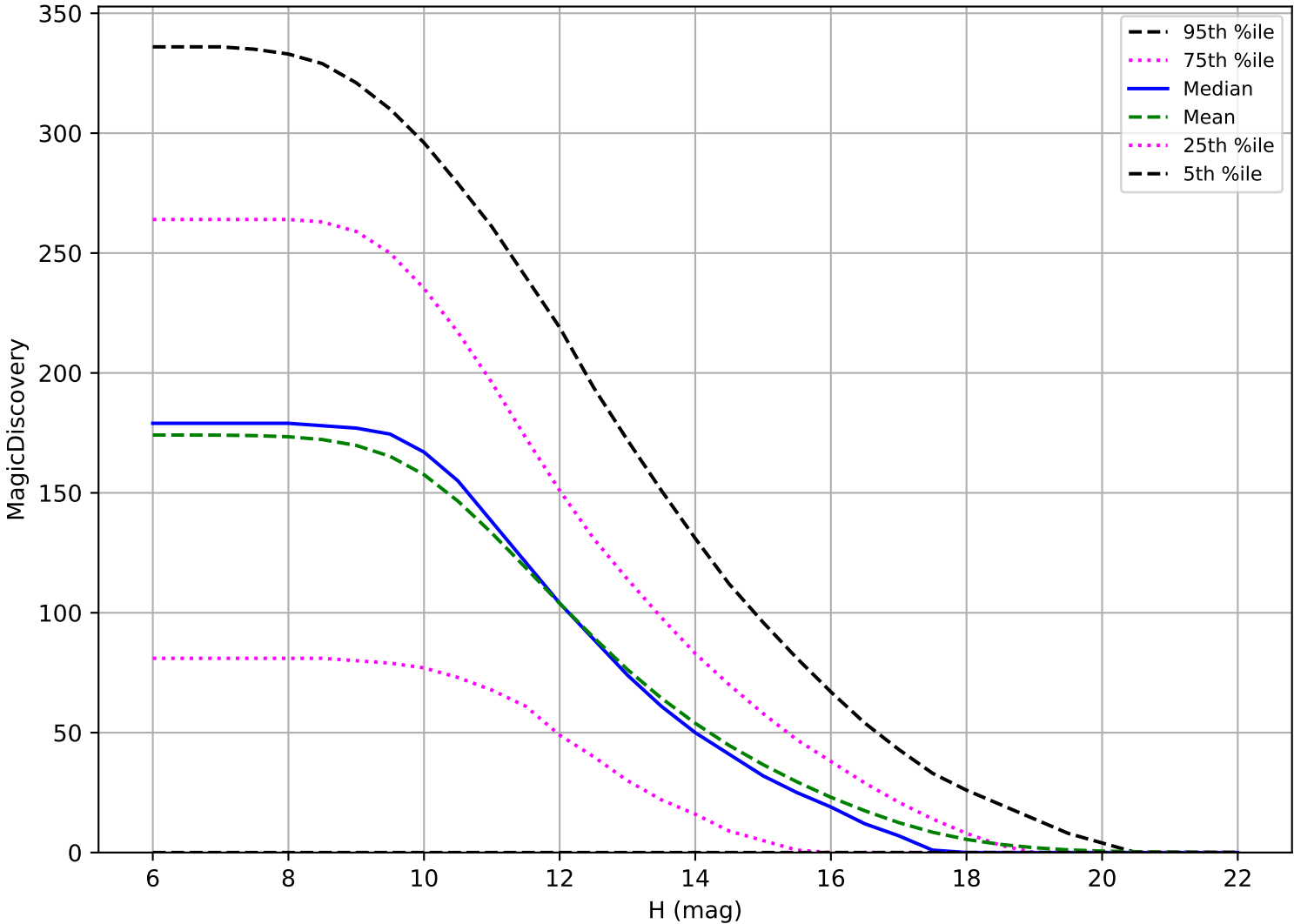
too_elab_2yr_r128_d3_ugrizy_v3.4_10yrs: OCC_r5 6 detections in 60 nights detection loss
