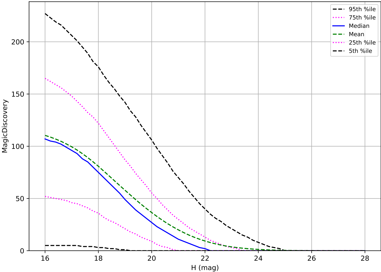
too_elab_2yr_r128_d3_ugrizy_v3.4_10yrs: NEO 6 detections in 60 nights detection loss
