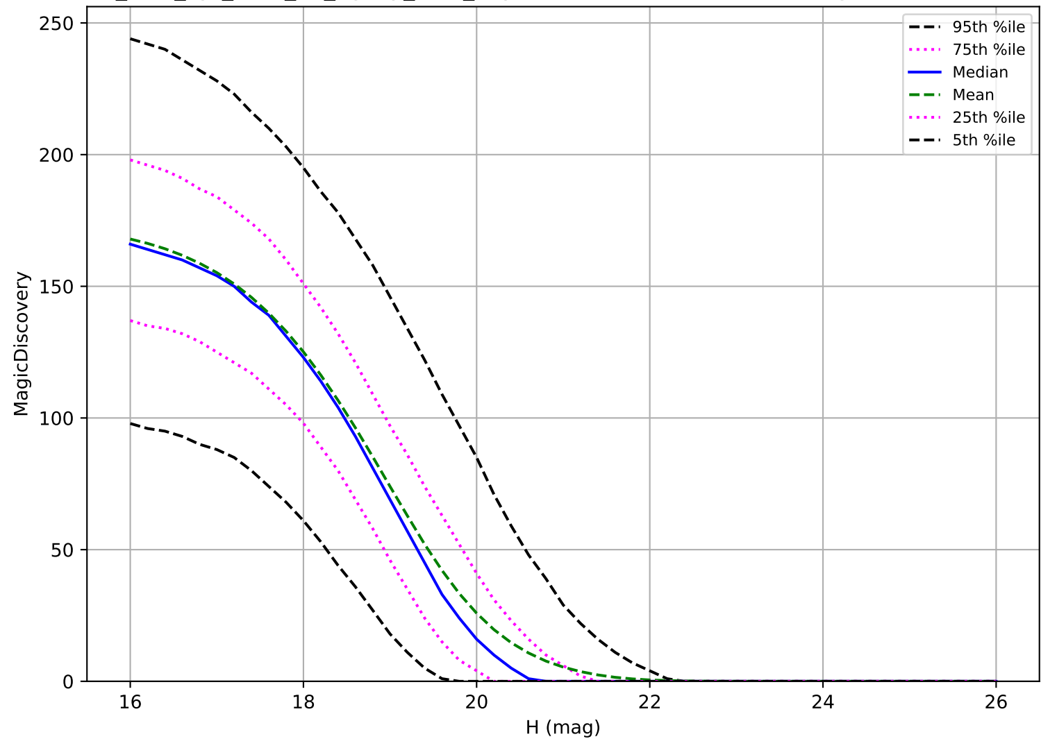
too_elab_2yr_r128_d3_ugrizy_v3.4_10yrs: MBA 6 detections in 60 nights detection loss
