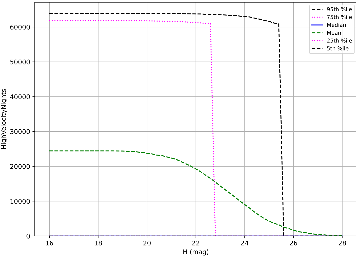
too_elab_2yr_r128_d3_ugrizy_v3.4_10yrs: PHA High velocity pair detection loss
