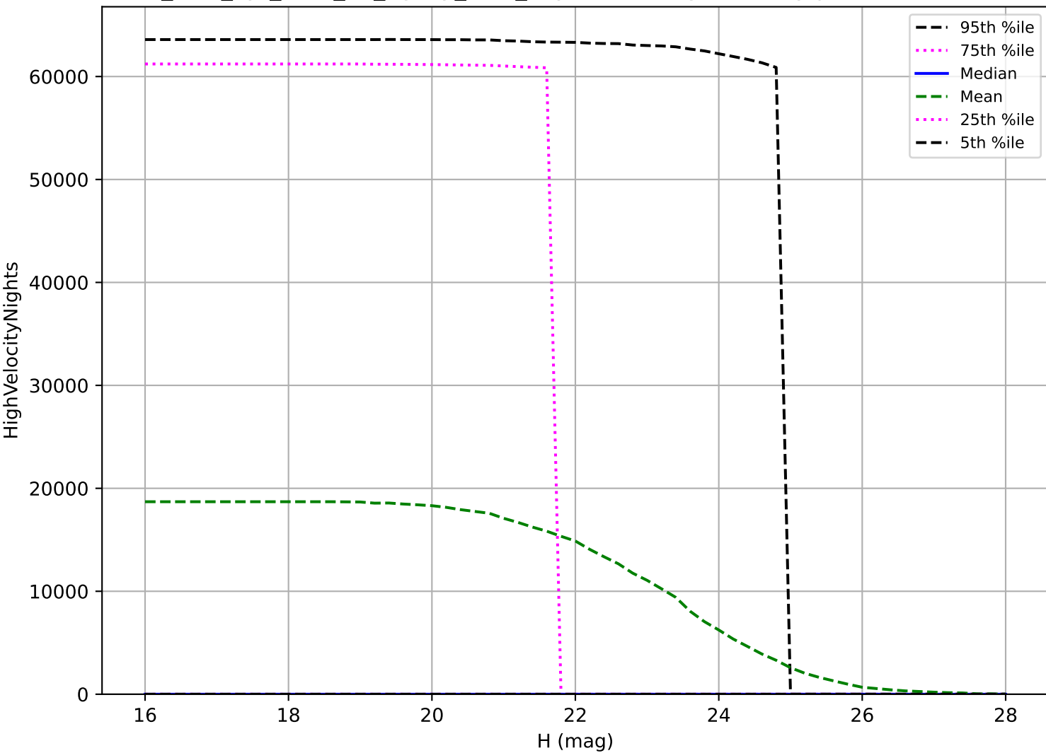
too_elab_2yr_r128_d3_ugrizy_v3.4_10yrs: NEO High velocity pair detection loss
