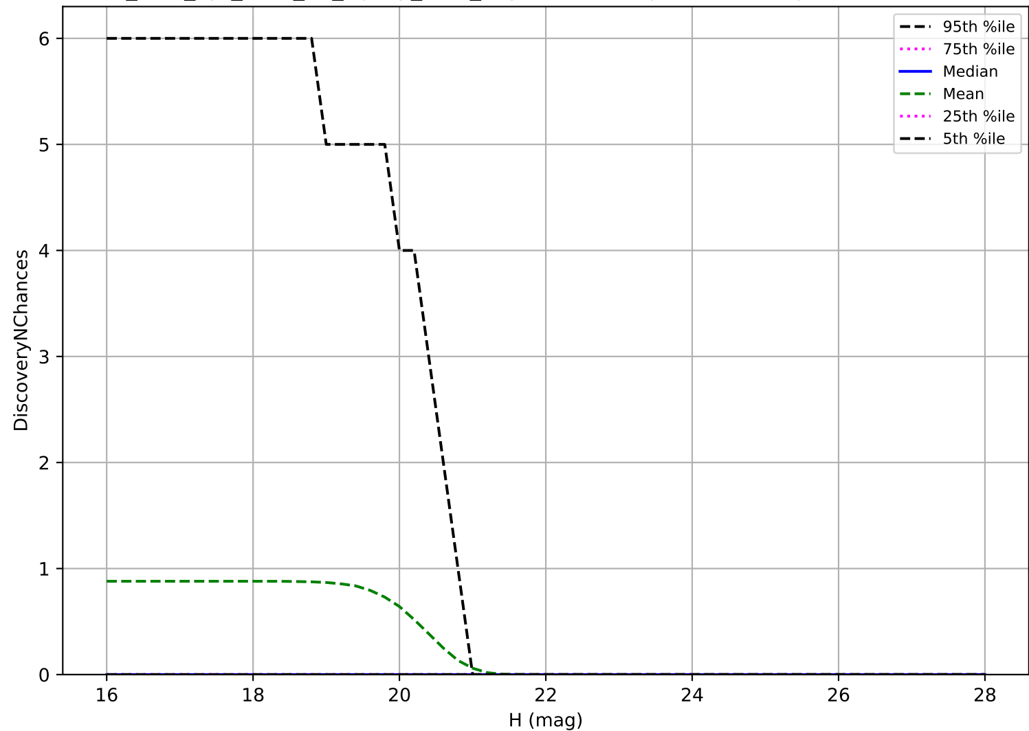
too_elab_2yr_r128_d3_ugrizy_v3.4_10yrs: Vatira 3 pairs in 15 nights detection loss
