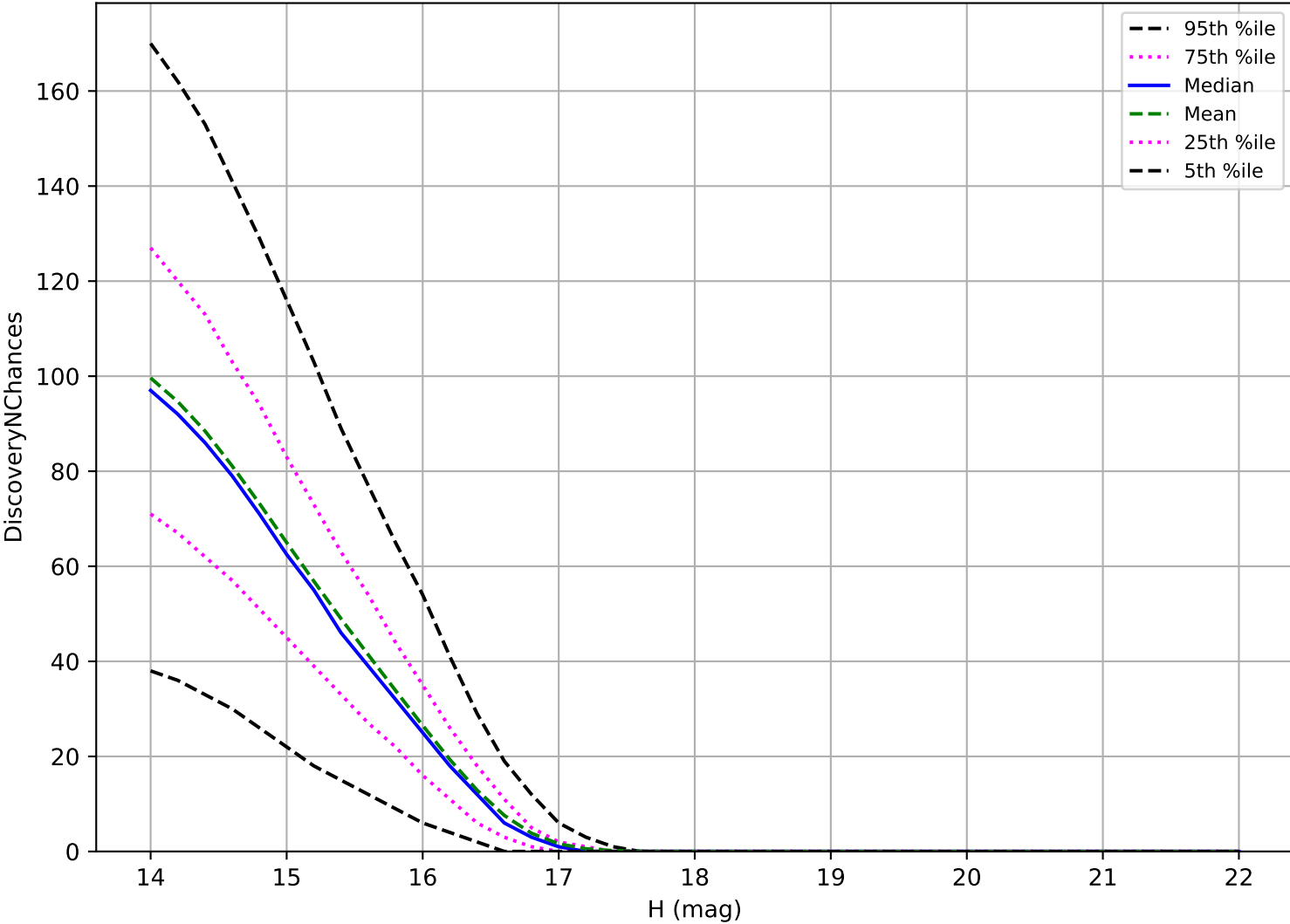
too_elab_2yr_r128_d3_ugrizy_v3.4_10yrs: Trojan 3 pairs in 15 nights detection loss
