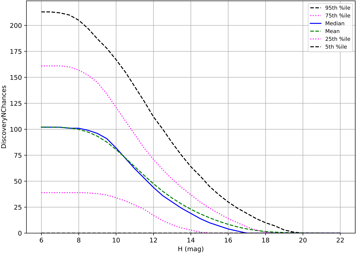
too_elab_2yr_r128_d3_ugrizy_v3.4_10yrs: OCC_r5 3 pairs in 15 nights detection loss
