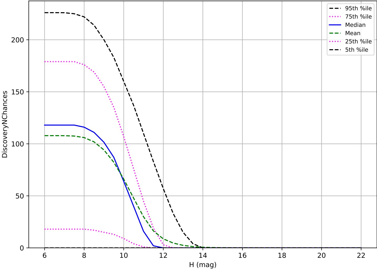
too_elab_2yr_r128_d3_ugrizy_v3.4_10yrs: OCC_r20 3 pairs in 15 nights detection loss
