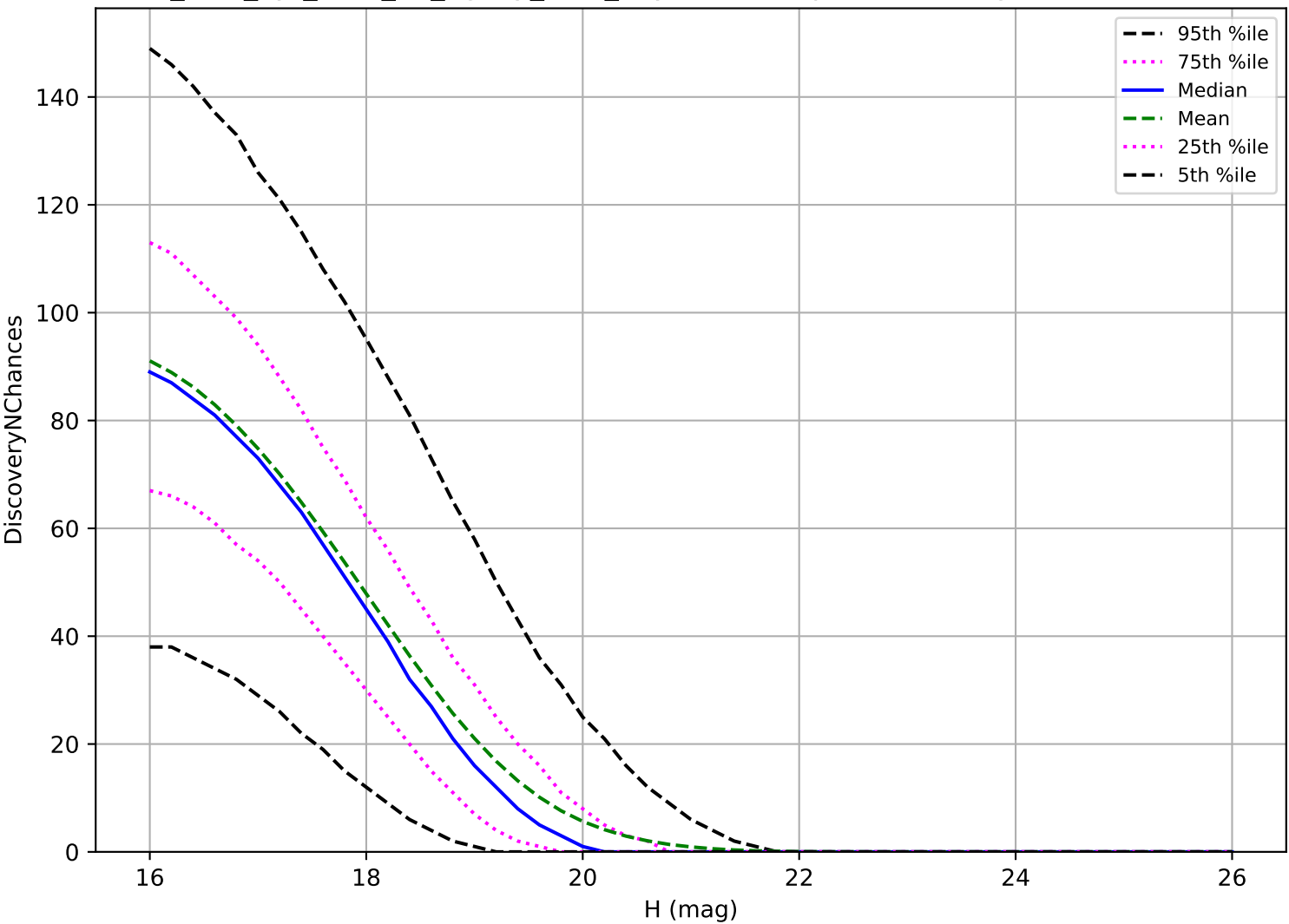
too_elab_2yr_r128_d3_ugrizy_v3.4_10yrs: MBA 3 pairs in 15 nights detection loss
