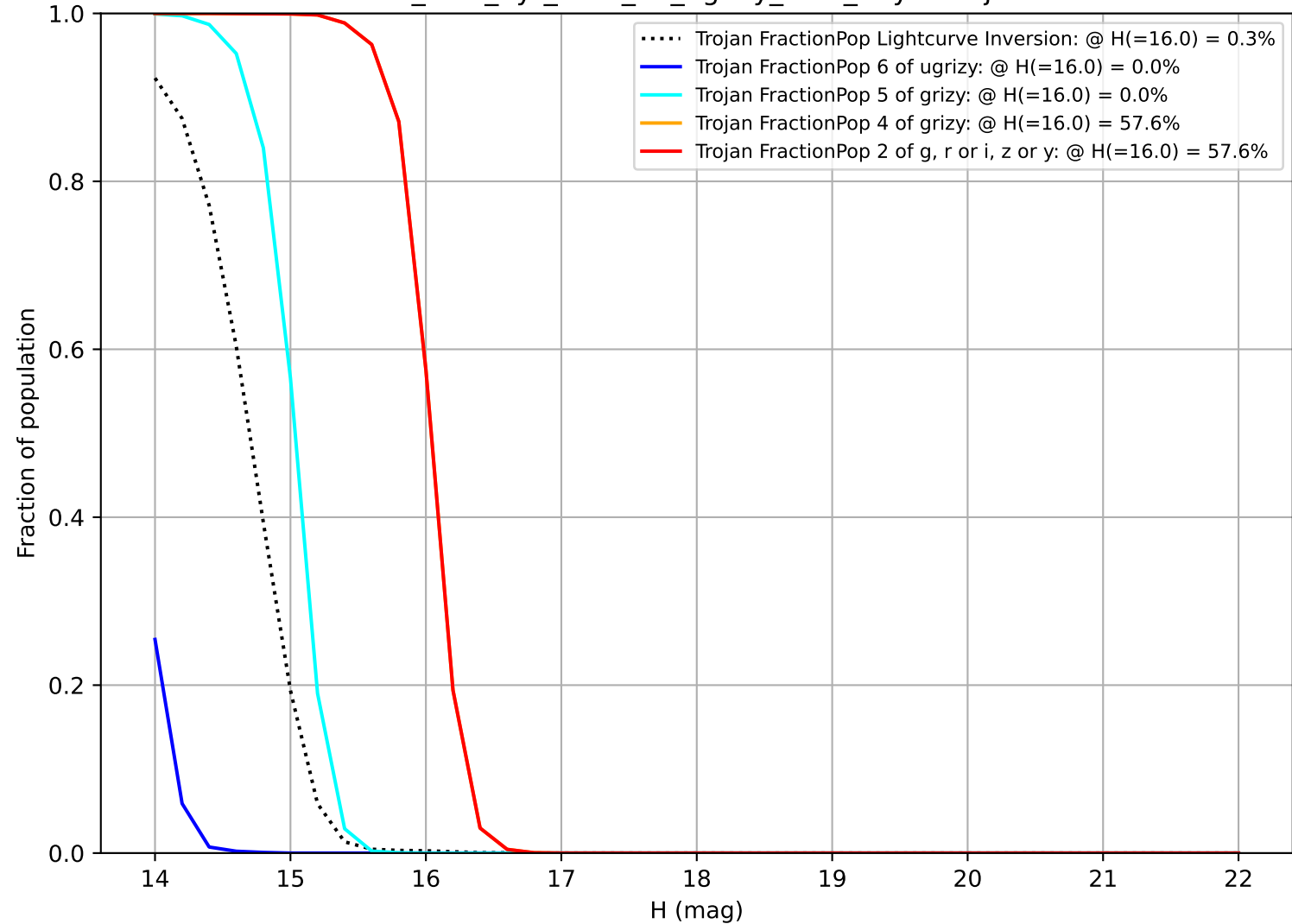
too_elab_2yr_r128_d3_ugrizy_v3.4_10yrs Trojan
