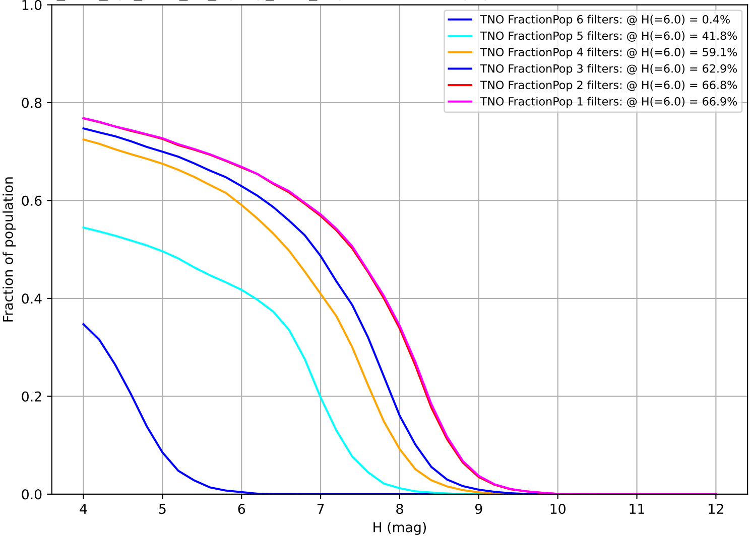
too_elab_2yr_r128_d3_ugrizy_v3.4_10yrs: Fraction of population with colors in X filters TNO
