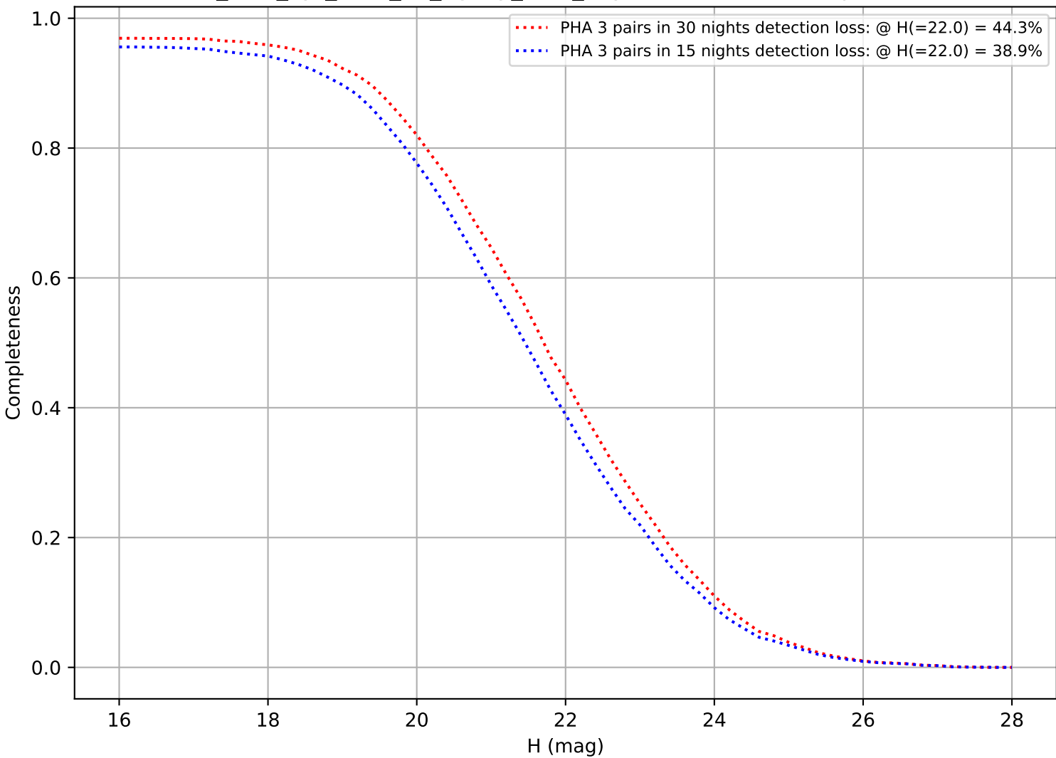
too_elab_2yr_r128_d3_ugrizy_v3.4_10yrs: DifferentialCompleteness
