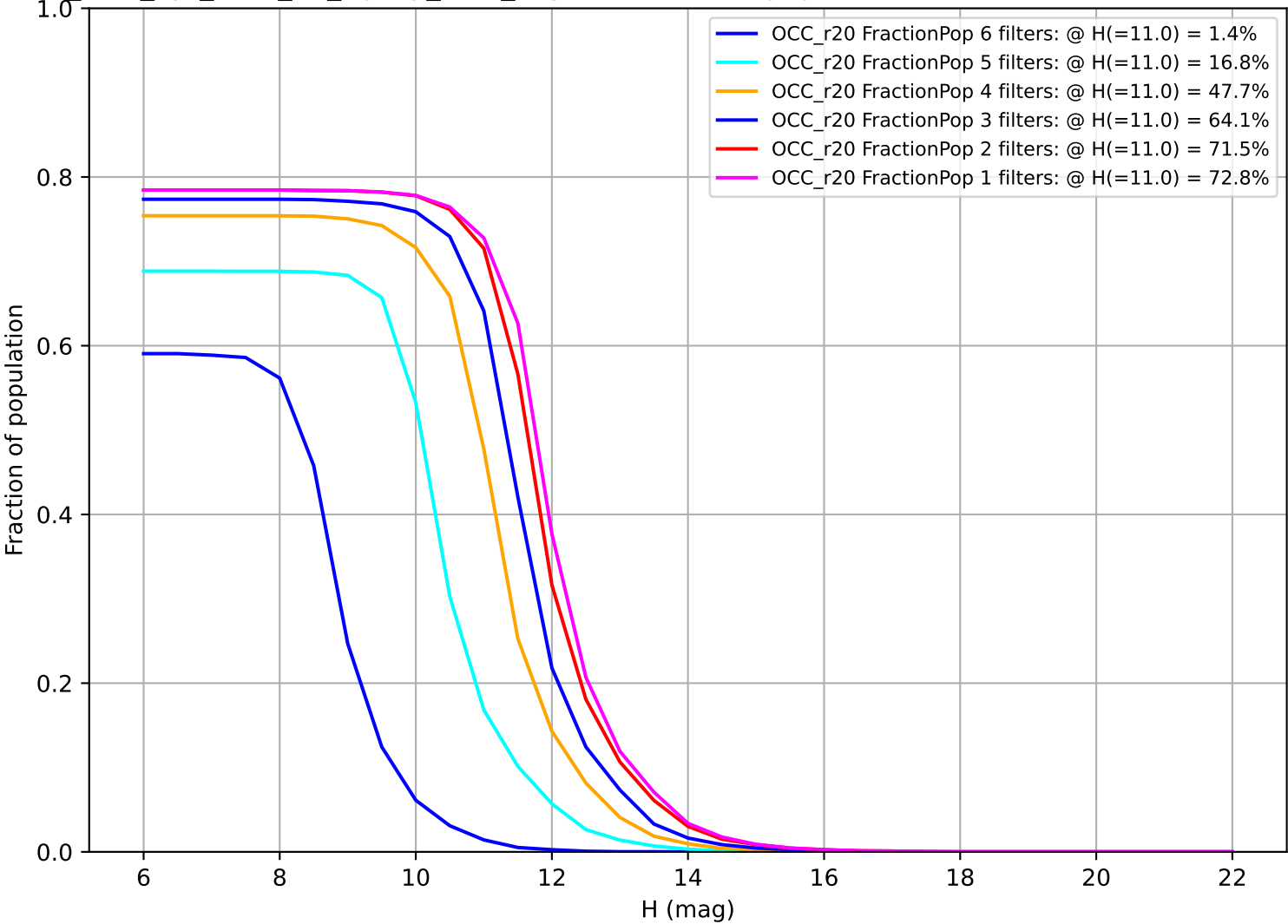
too_elab_2yr_r128_d3_ugrizy_v3.4_10yrs: Fraction of population with colors in X filters OCC_r20
