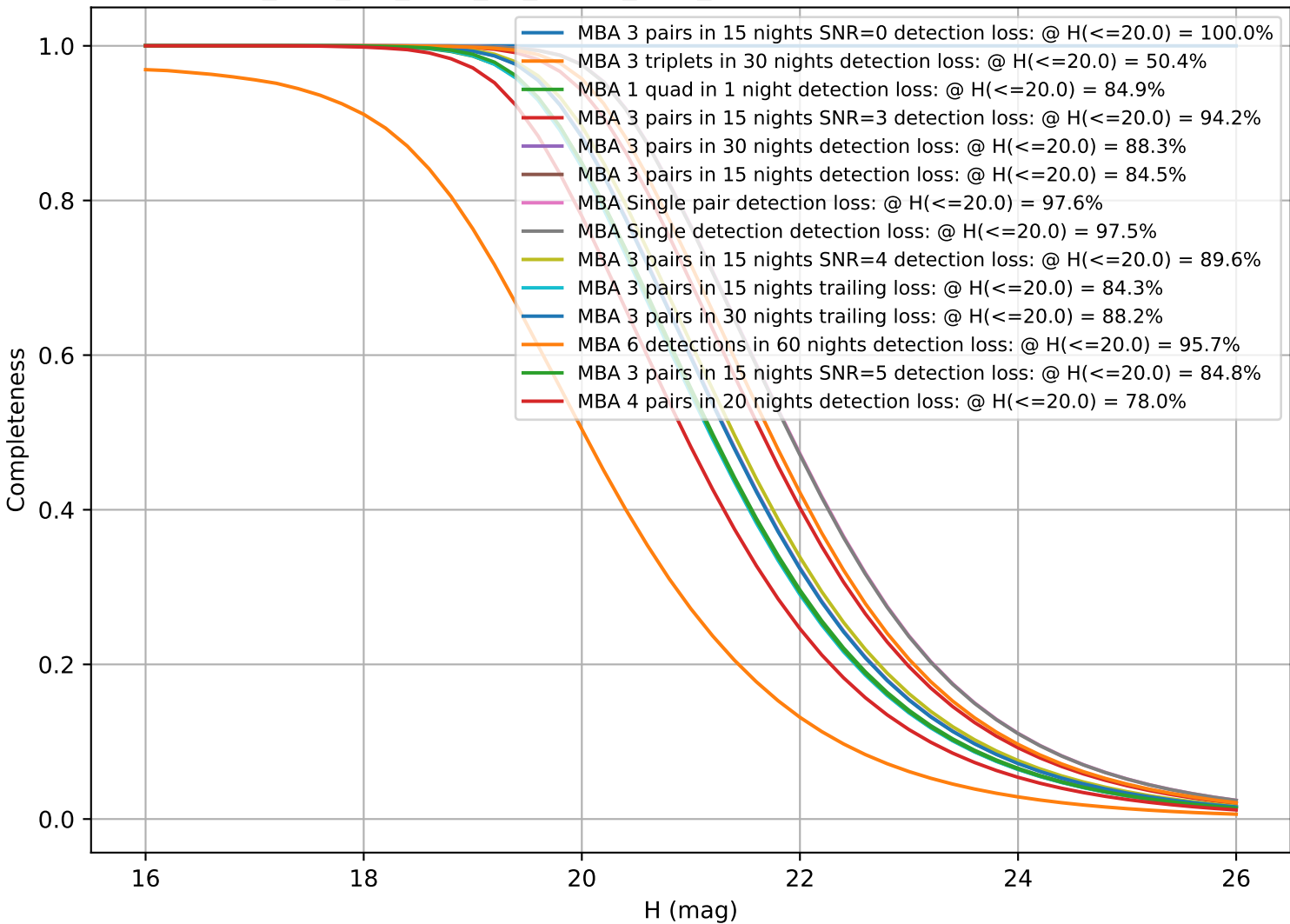
too_elab_2yr_r128_d3_ugrizy_v3.4_10yrs: CumulativeCompleteness
