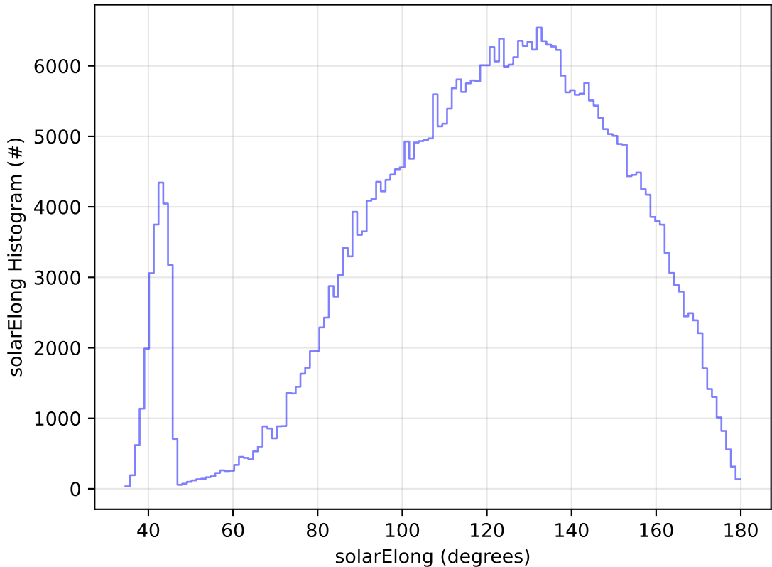
too_elab_2yr_r128_d3_ugrizy_v3.4_10yrs WFD z band: solarElong Histogram
