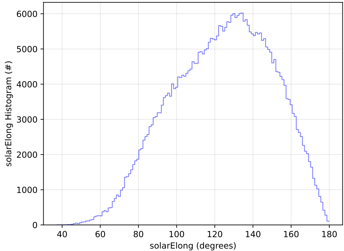
too_elab_2yr_r128_d3_ugrizy_v3.4_10yrs WFD y band: solarElong Histogram
