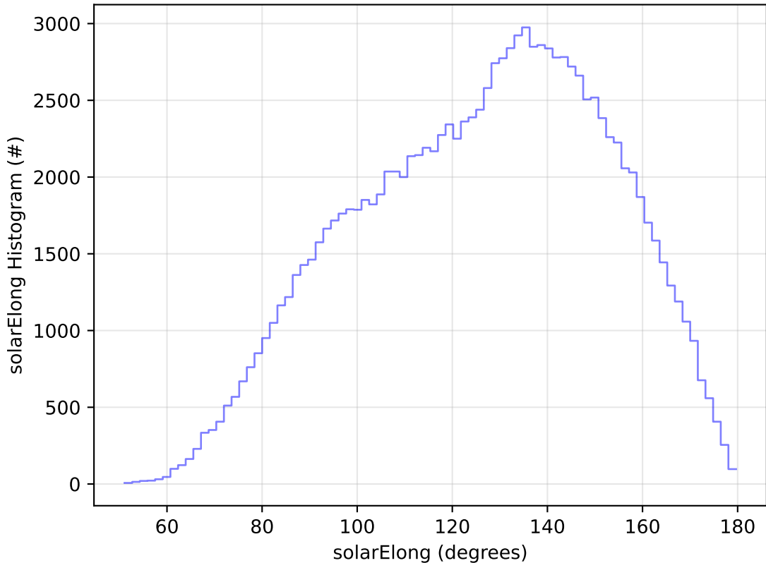
too_elab_2yr_r128_d3_ugrizy_v3.4_10yrs WFD u band: solarElong Histogram
