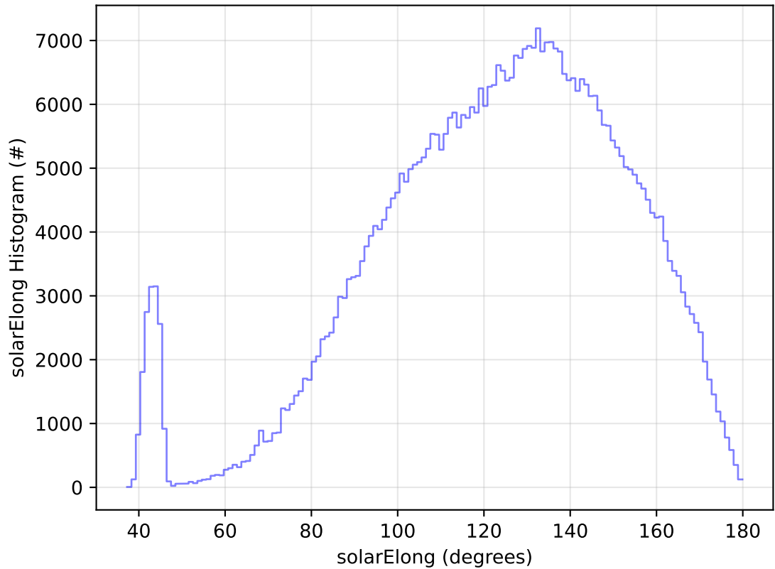
too_elab_2yr_r128_d3_ugrizy_v3.4_10yrs WFD r band: solarElong Histogram
