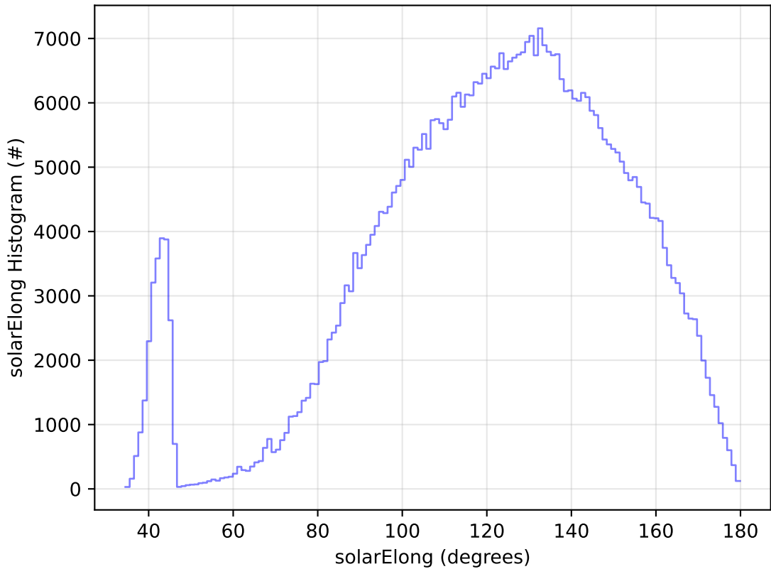
too_elab_2yr_r128_d3_ugrizyv3.4_10yrs WFD i band: solarElong Histogram
