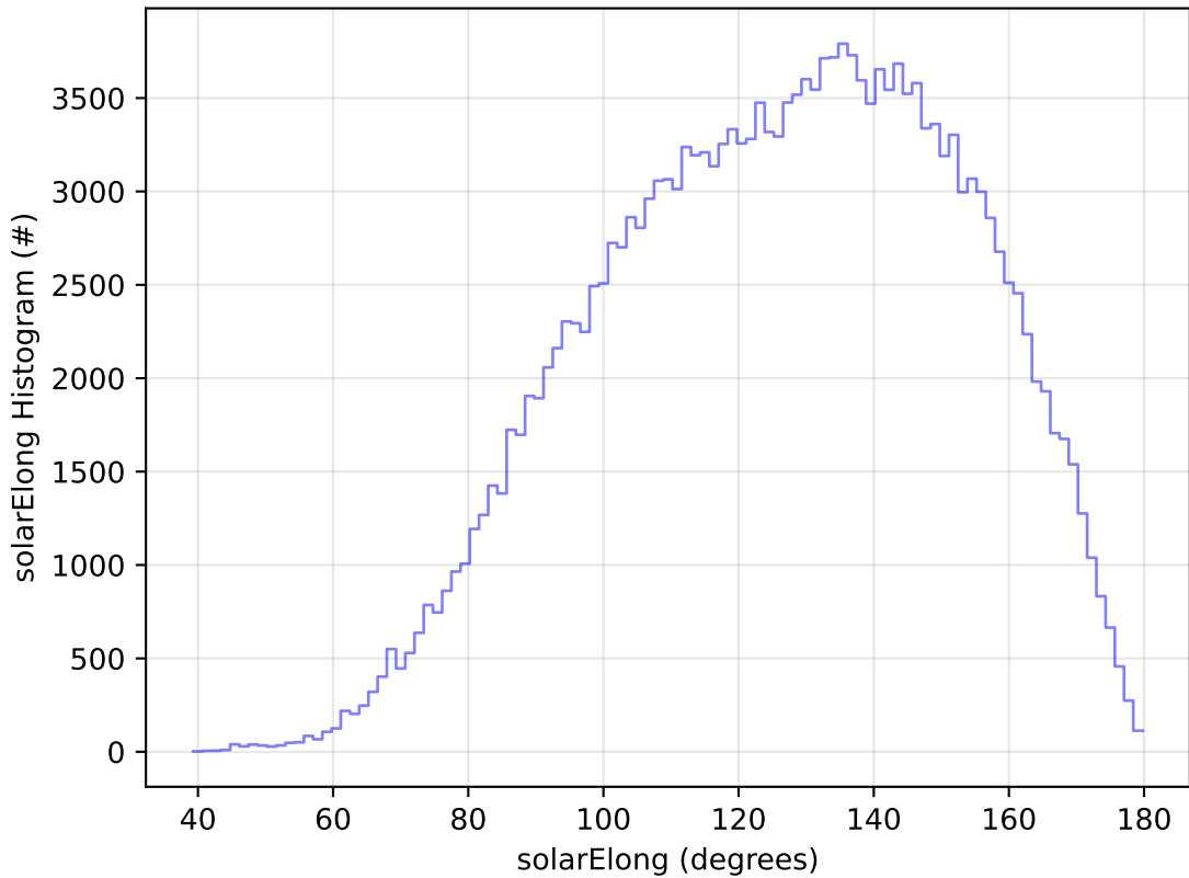
too_elab_2yr_r128_d3_ugrizy_v3.4_10yrs WFD g band: solarElong Histogram
