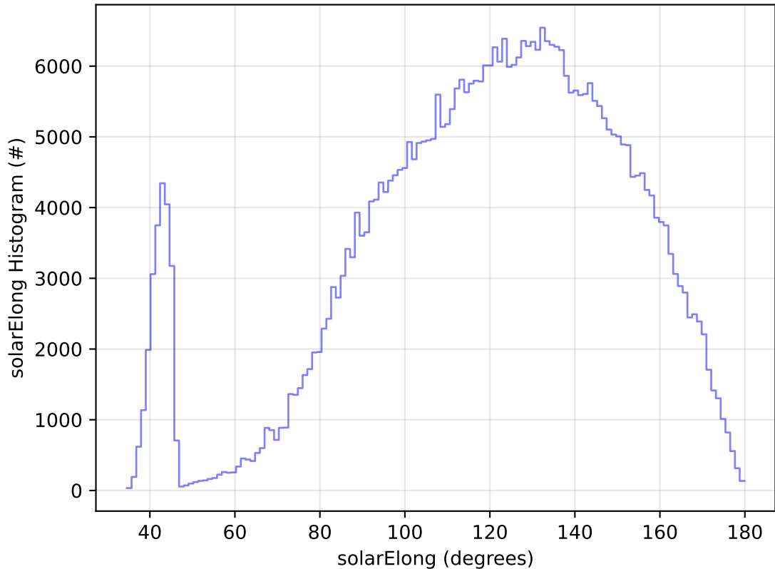
too_elab_2yr_r128_d3_ugrizy_v3.4_10yrs All sky z band: solarElong Histogram
