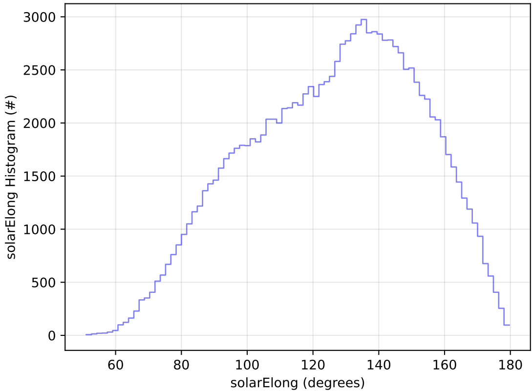
too_elab_2yr_r128_d3_ugrizy_v3.4_10yrs All sky u band: solarElong Histogram
