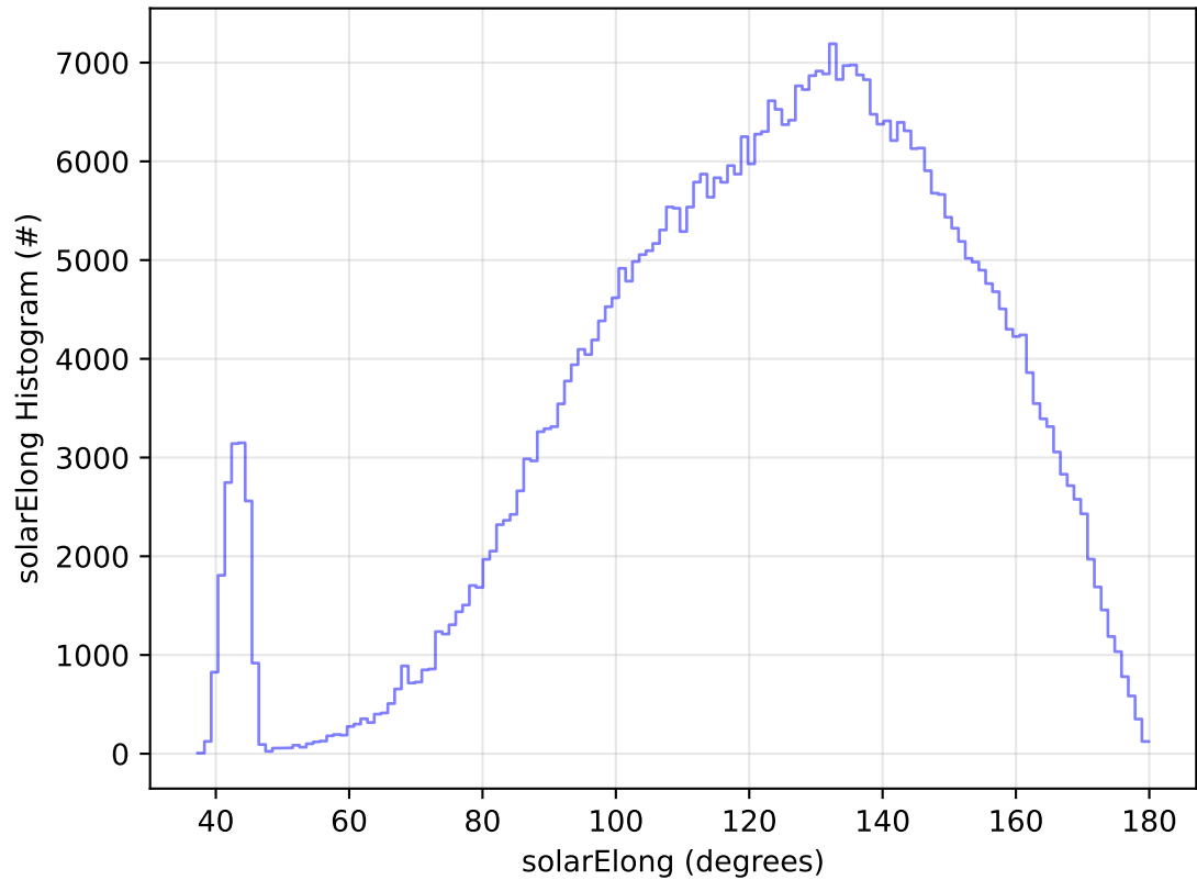
too_elab_2yr_r128_d3_ugrizy_v3.4_10yrs All sky r band: solarElong Histogram
