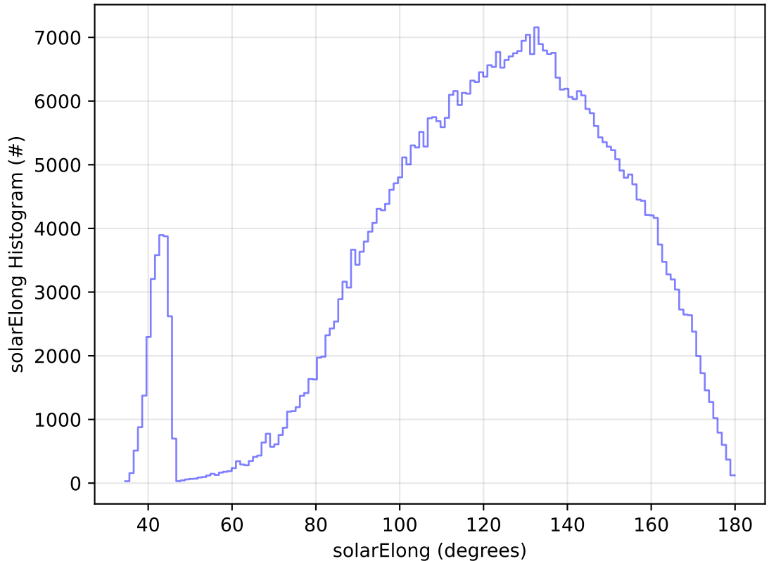
too_elab_2yr_r128_d3_ugrizy_v3.4_10yrs All sky i band: solarElong Histogram
