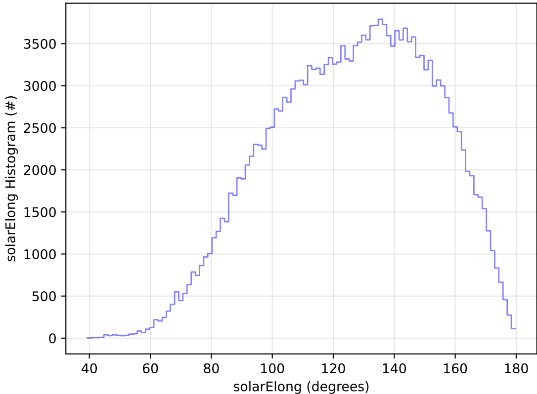
too_elab_2yr_r128_d3_ugrizy_v3.4_10yrs All sky g band: solarElong Histogram
