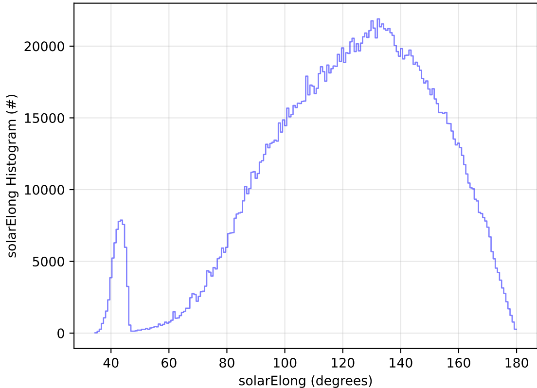
too_elab_2yr_r128_d3_ugrizy_v3.4_10yrs All sky all bands: solarElong Histogram
