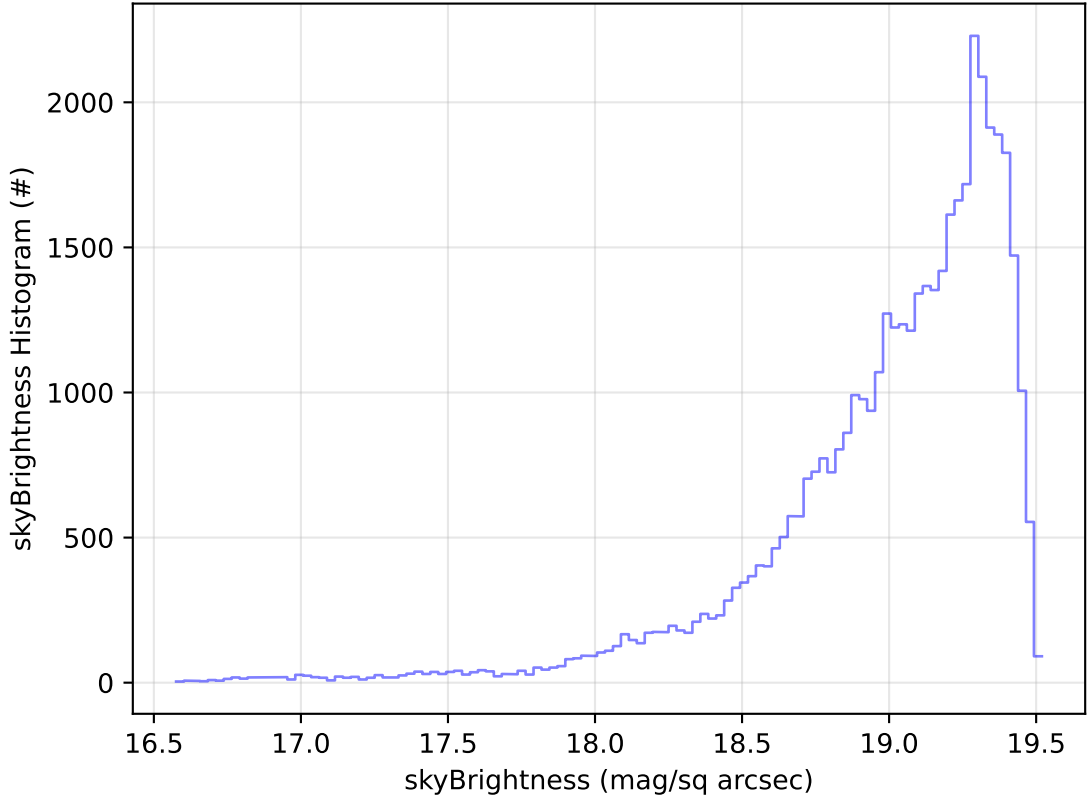
too_elab_2yr_r128_d3_ugrizy_v3.4_10yrs Yr 1 z band: skyBrightness Histogram
