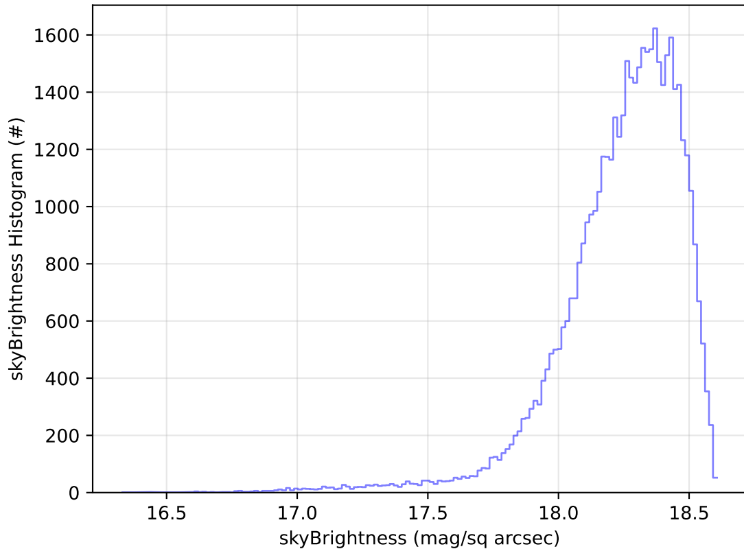
too_elab_2yr_r128_d3_ugrizy_v3.4_10yrs Yr 1 y band: skyBrightness Histogram
