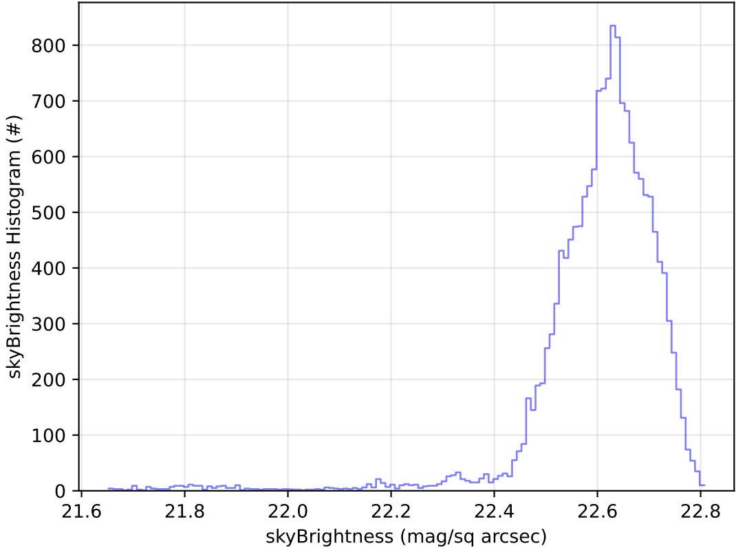
too_elab_2yr_r128_d3_ugrizy_v3.4_10yrs Yr 1 u band: skyBrightness Histogram
