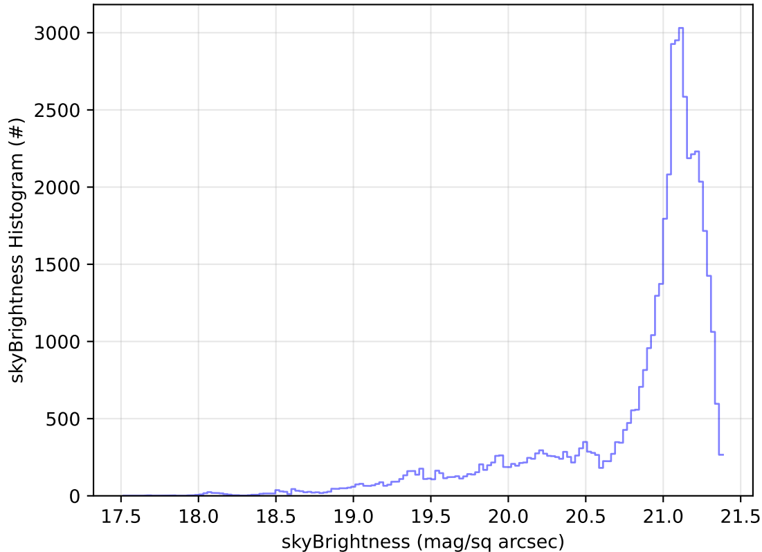
too_elab_2yr_r128_d3_ugrizy_v3.4_10yrs Yr 1 r band: skyBrightness Histogram
