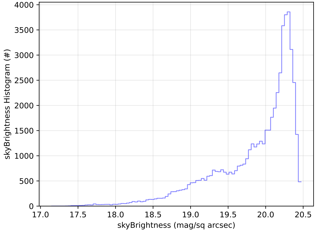
too_elab_2yr_r128_d3_ugrizy_v3.4_10yrs Yr 1 i band: skyBrightness Histogram
