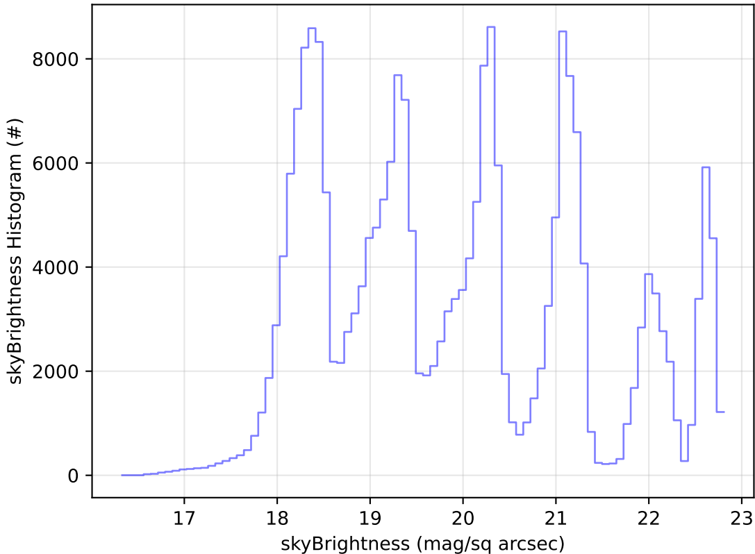
too_elab_2yr_r128_d3_ugrizy_v3.4_10yrs Yr 1 all bands: skyBrightness Histogram
