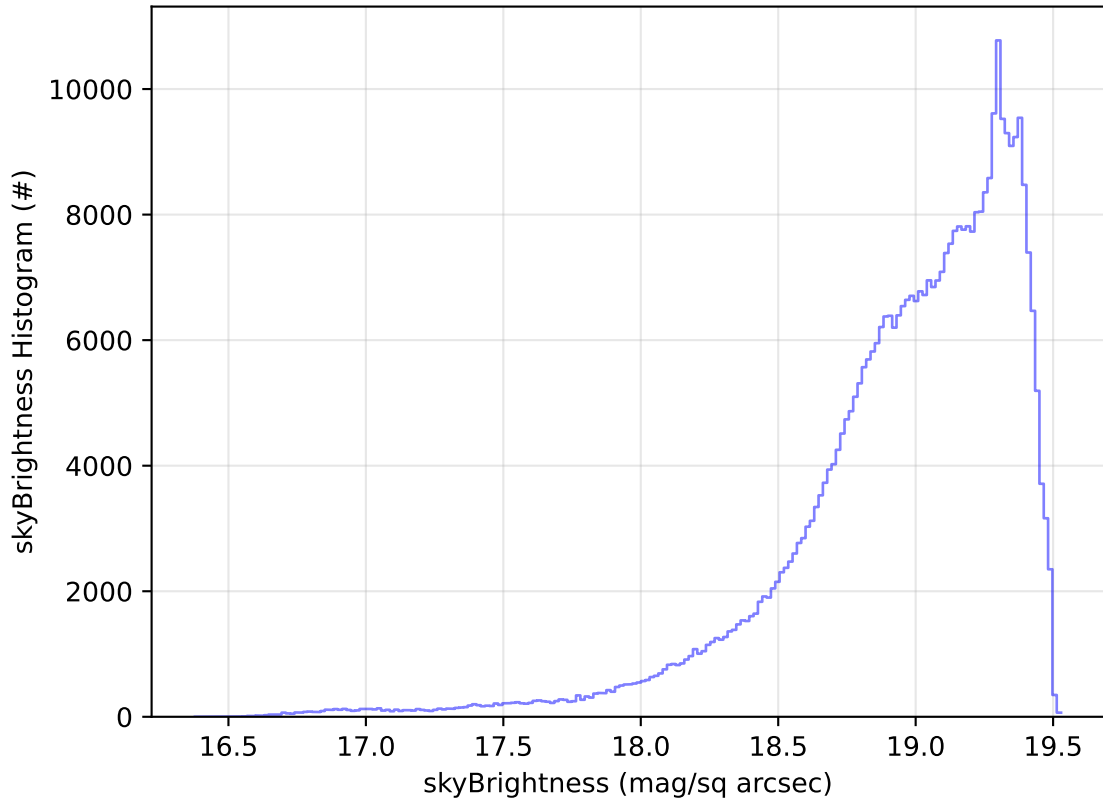
too_elab_2yr_r128_d3_ugrizy_v3.4_10yrs WFD z band: skyBrightness Histogram
