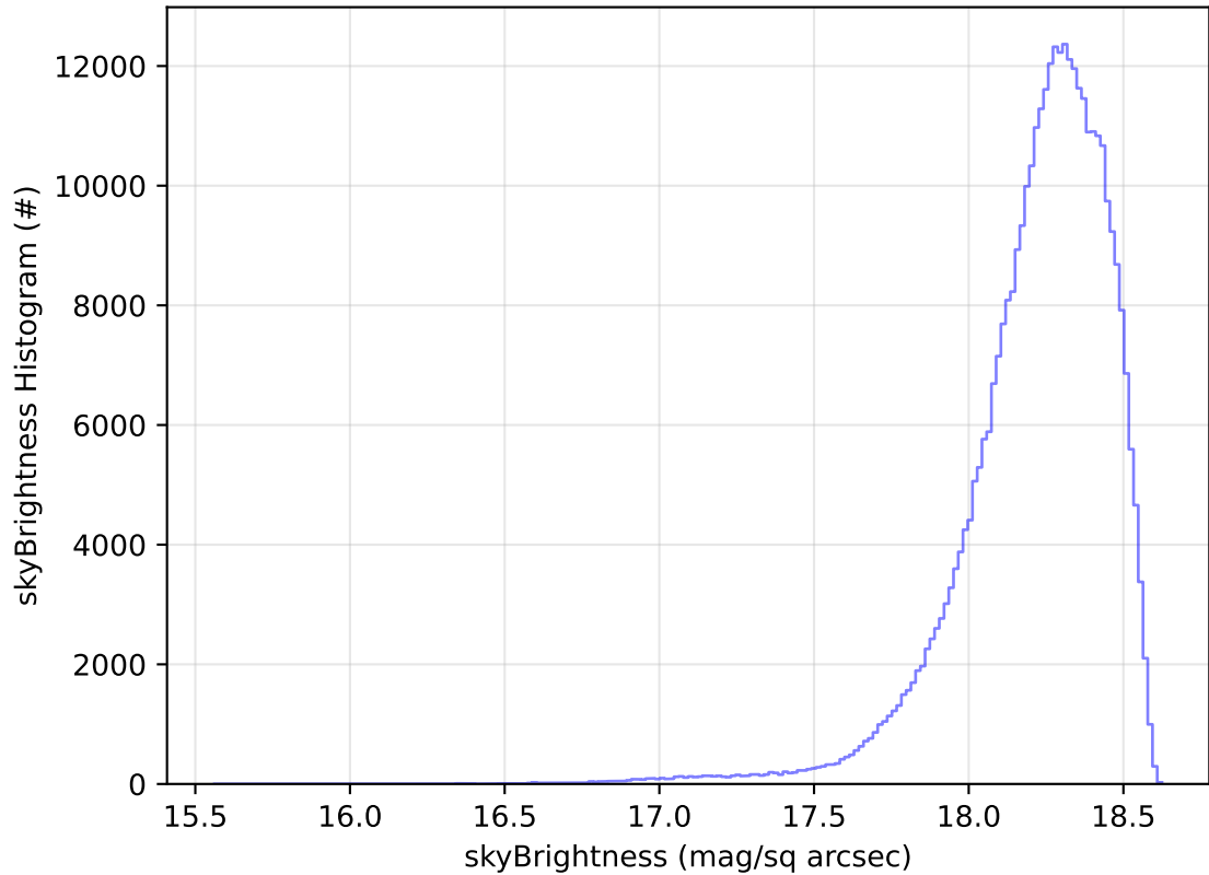
too_elab_2yr_r128_d3_ugrizy_v3.4_10yrs WFD y band: skyBrightness Histogram
