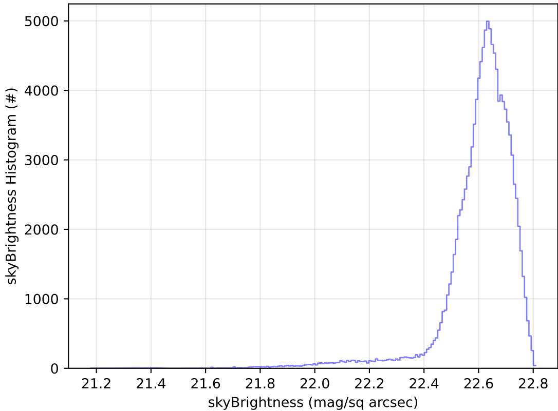
too_elab_2yr_r128_d3_ugrizy_v3.4_10yrs WFD u band: skyBrightness Histogram
