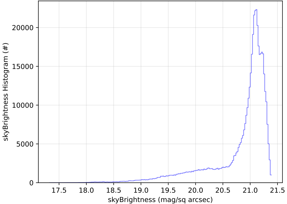
too_elab_2yr_r128_d3_ugrizy_v3.4_10yrs WFD r band: skyBrightness Histogram
