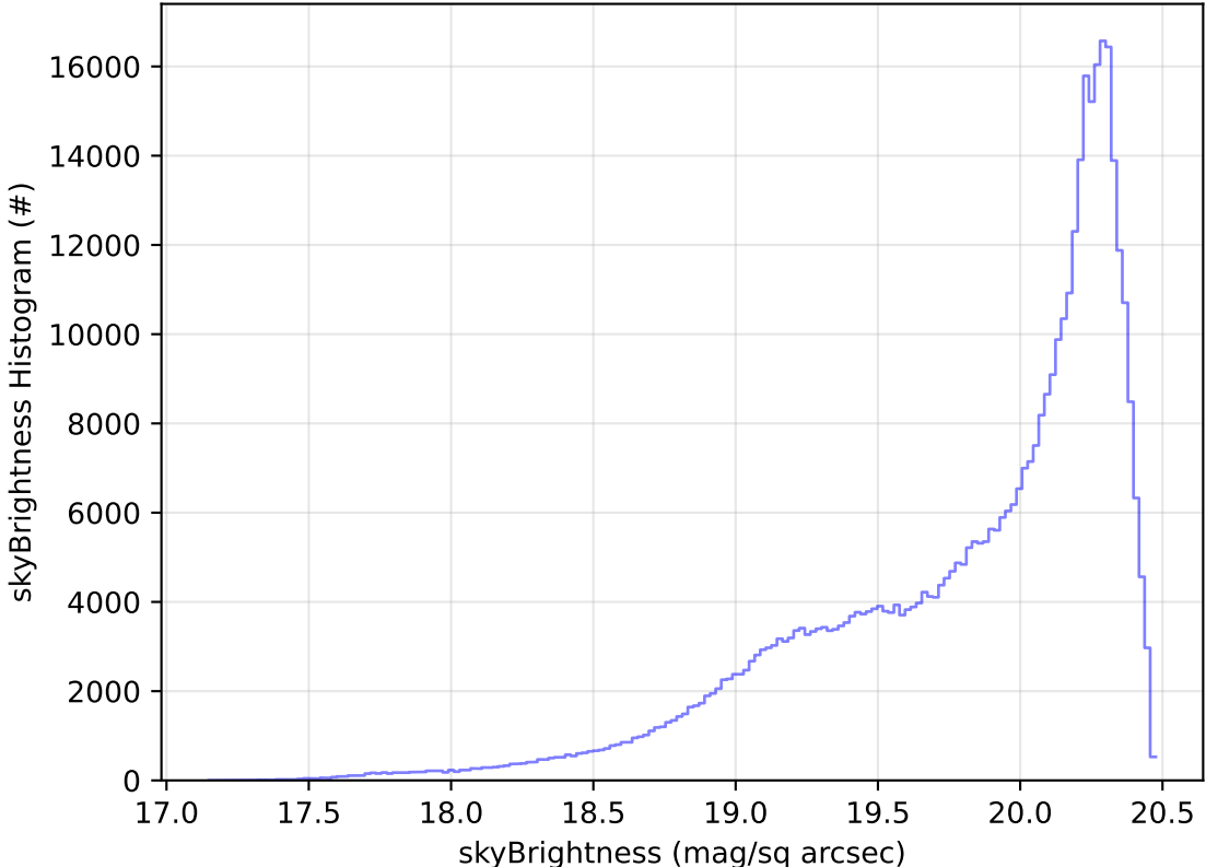
too_elab_2yr_r128_d3_ugrizy_v3.4_10yrs WFD i band: skyBrightness Histogram
