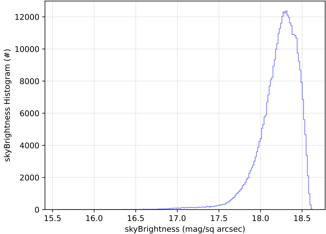
too_elab_2yr_r128_d3_ugrizy_v3.4_10yrs All sky y band: skyBrightness Histogram
