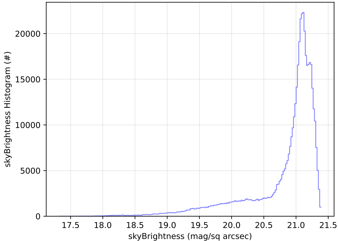
too_elab_2yr_r128_d3_ugrizy_v3.4_10yrs All sky r band: skyBrightness Histogram
