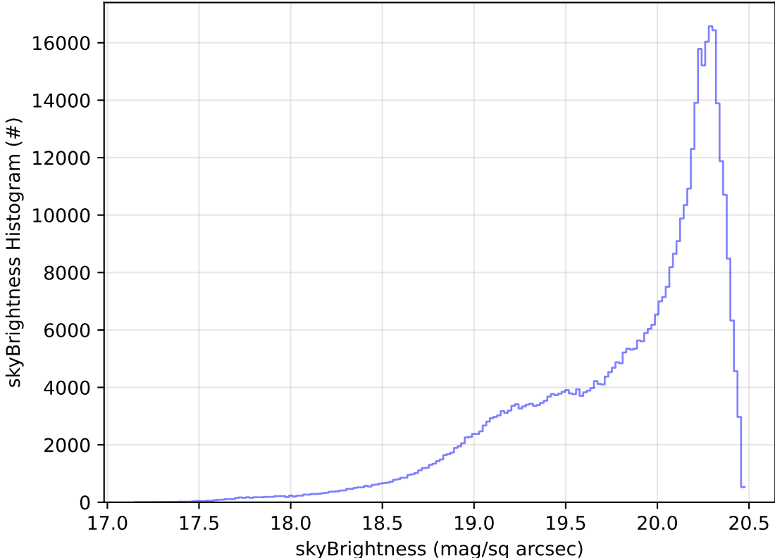
too_elab_2yr_r128_d3_ugrizy_v3.4_10yrs All sky i band: skyBrightness Histogram
